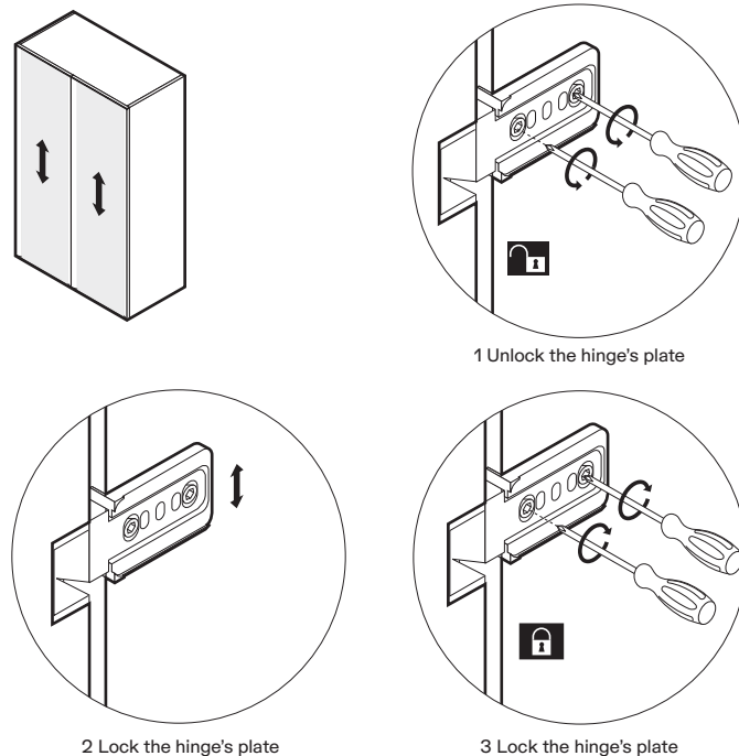
2 Lock the hinge's plate
