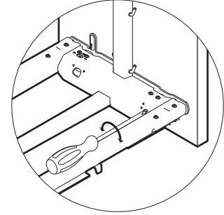
Adjust the screws indicated
