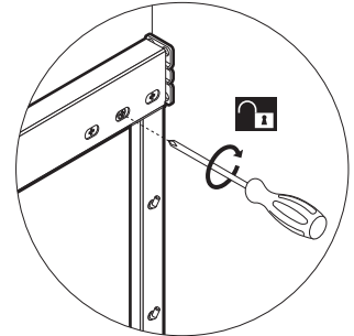
1 Unlock the system,
