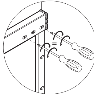
2 Adjust the screws in the same rotation direction
